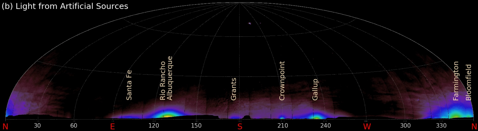
Figure 9: Panoramic night sky images from the Water Tank site on 01/30/2003. (a) Observed night sky. (b) Light from artificial sources.
