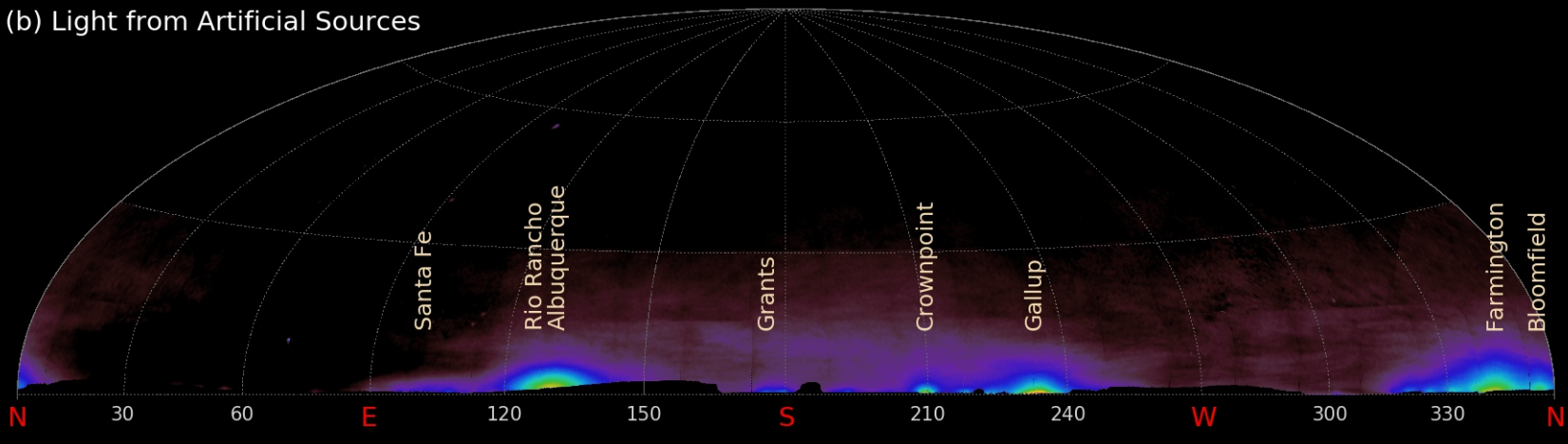
Figure 7: Panoramic night sky images from the Water Tank site on 10/13/2001. (a) Observed night sky. (b) Light from artificial sources.
